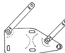
Hood hinge and props mount to steel structure
